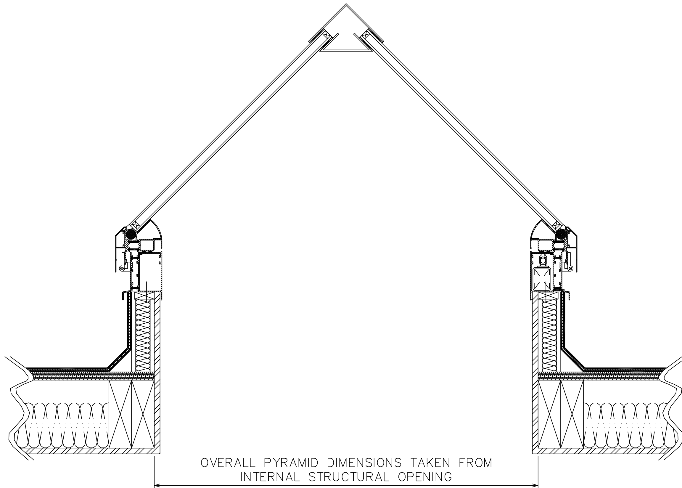
Section Through Upstand/Framework Construction
