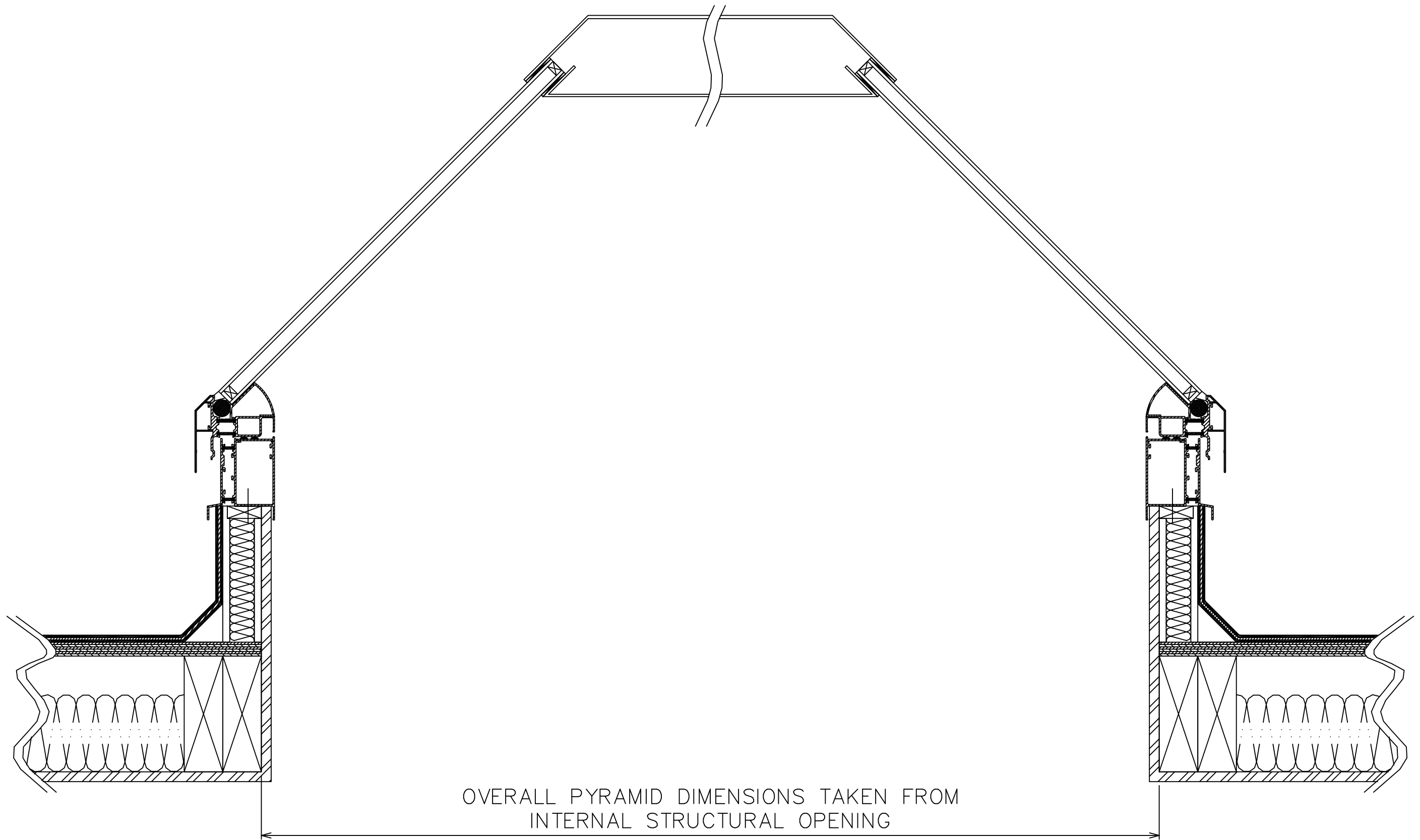
Section Through Upstand/Framework Construction
